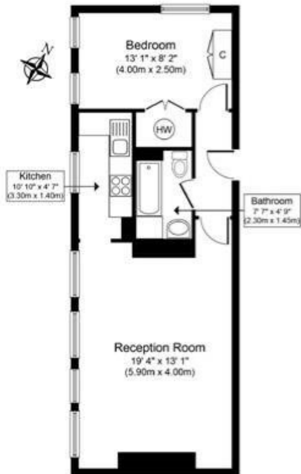
THE CLOISTERS, E1 TOTAL APPROX FLOORPLAN AREA 512 SQ.FT (47.6 SQ.M) FOURTH FLOOR
